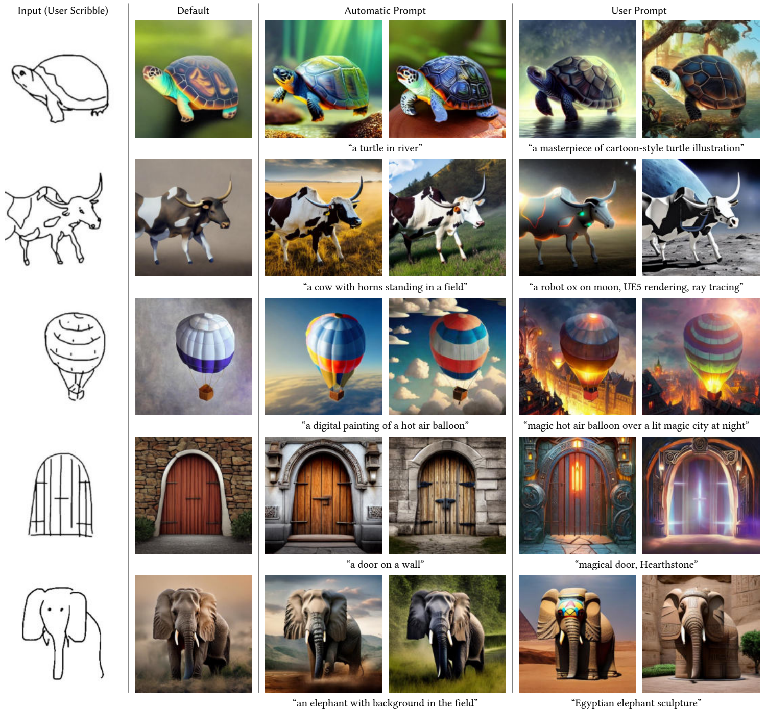
Figure 6: Controlling Stable Diffusion with Human scribbles. The “automatic prompts” are generated by BLIP based on the default result images without using user prompts. These scribbles are from [58].
