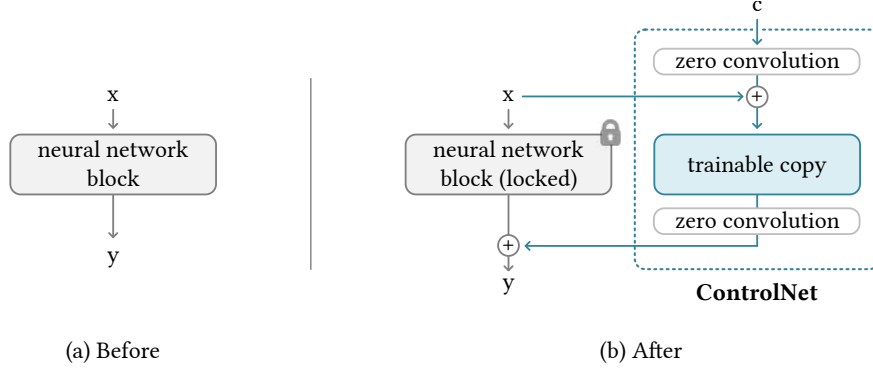
Figure 2: ControlNet. We show the approach to apply a ControlNet to an arbitrary neural network block. The x, y are deep features in neural networks. The “+” refers to feature addition. The “ c ” is an extra condition that we want to add to the neural network. The “zero convolution” is an 1 \times 1 convolution layer with both weight and bias initialized as zeros.
