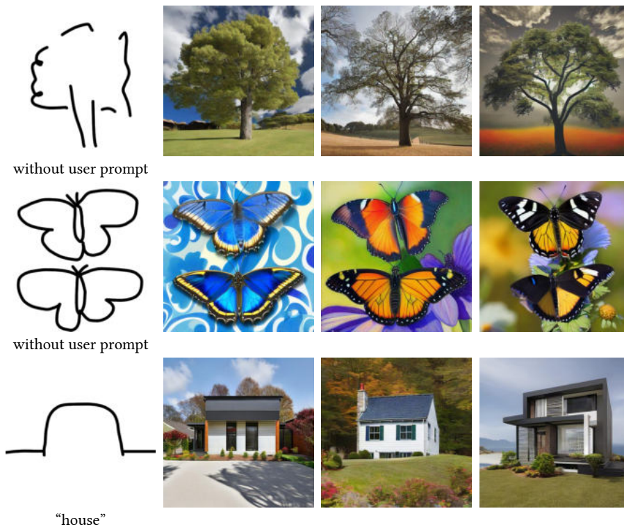
Figure 27: Coarse-level control. When users do not want their input shape to be preserved in the images, we can simply replace the last 50% diffusion iterations with standard SD without ControlNet. The resulting effect is similar to image retrieval but those images are generated.
